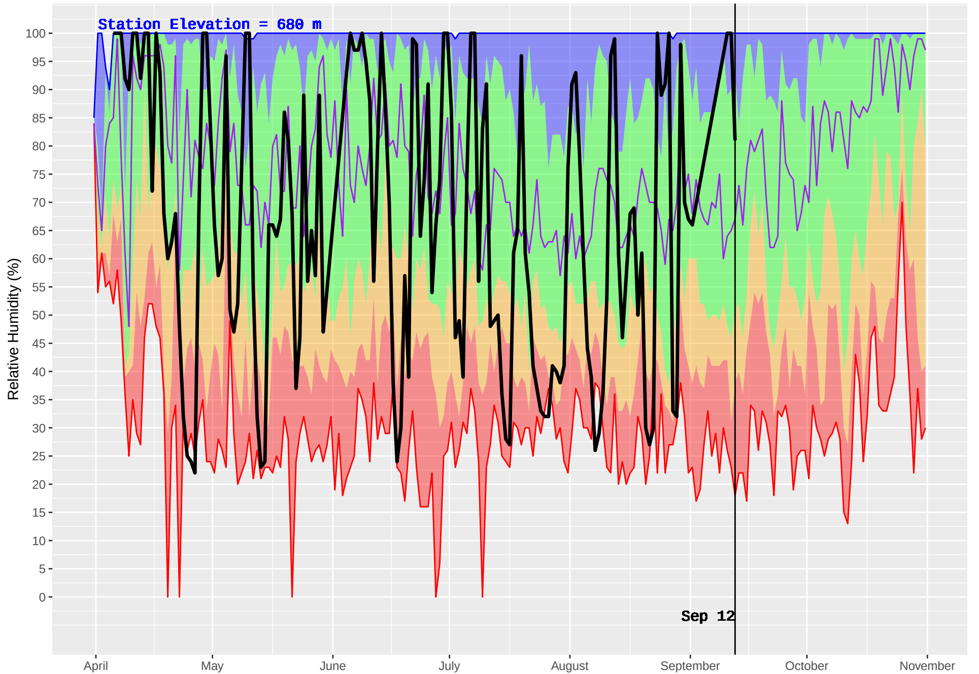
SUMMIT (11) : Historical (1985–2016) and Current (2018) Daily Relative Humidity
